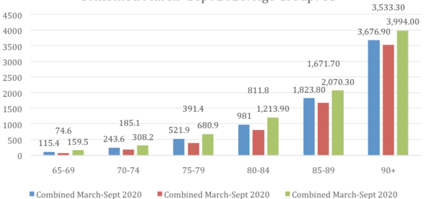
All Deaths Involving Covid 19 - Rates per 100,000 Combined March- Sept 2020. Age Group: 65+
